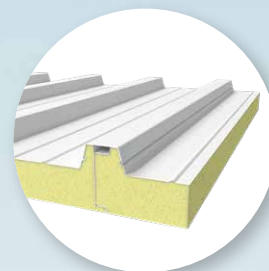
Option panneaux toiture aluminium 96mm 96mm aluminium roof panel option
