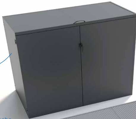
COFFRE XL 2000x1000x1400mm
