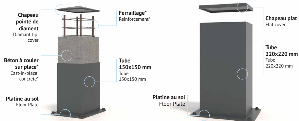
Section 150x150 mm À sceller | To be anchored
